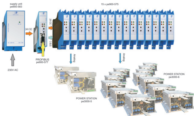
Example: power pack, pe900-577 and pe900-575 D/A interfaces for 15 analog POWER STATIONS
