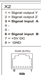
BUS output
